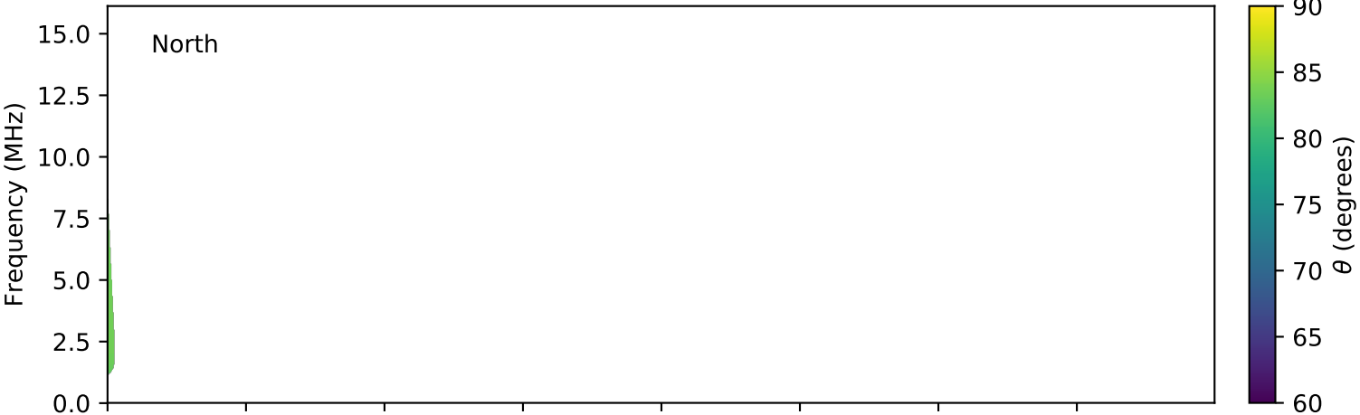
expres_cassini_jupiter_europa_isaac_lossc-wid1deg_3kev_20020813_v01.cdf
