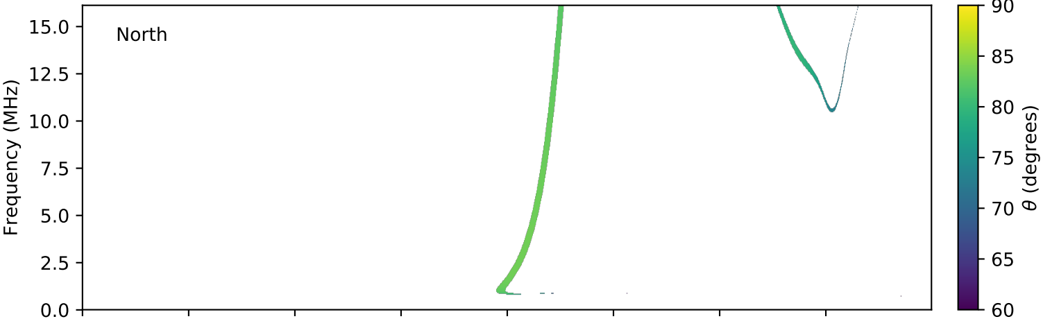
expres_cassini_jupiter_europa_isaac_lossc-wid1deg_3kev_20020811_v01.cdf
