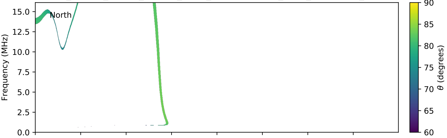
expres_cassini_jupiter_europa_isaac_lossc-wid1deg_3kev_20020809_v01.cdf
