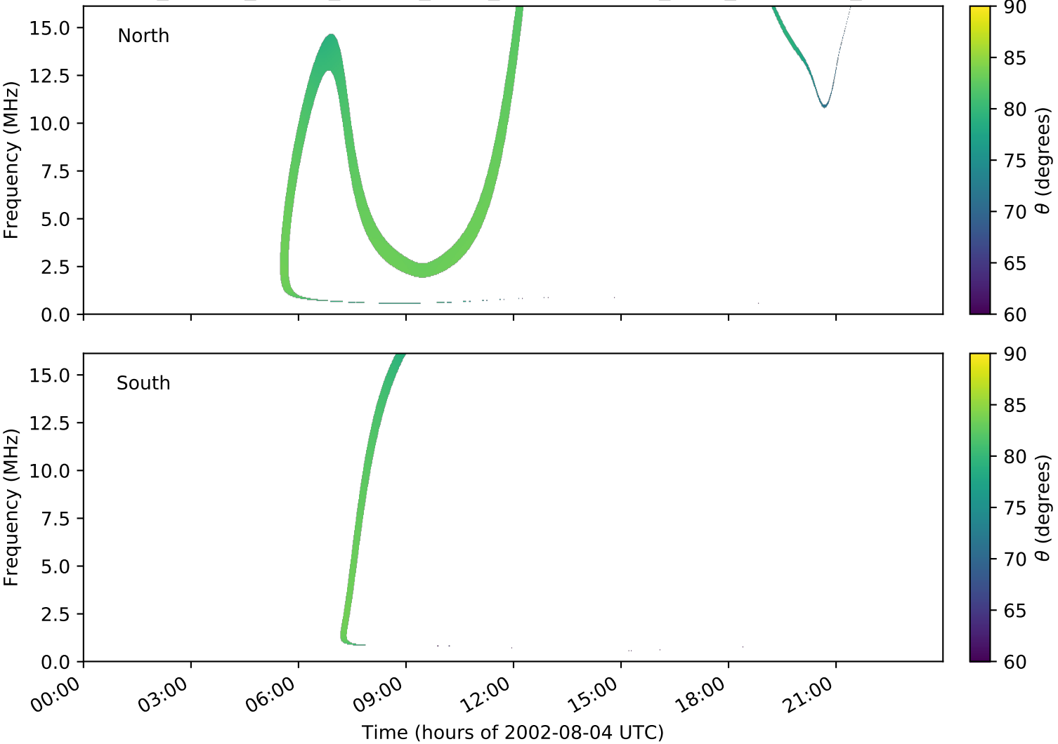
expres_cassini_jupiter_europa_isaac_lossc-wid1deg_3kev_20020804_v01.cdf
