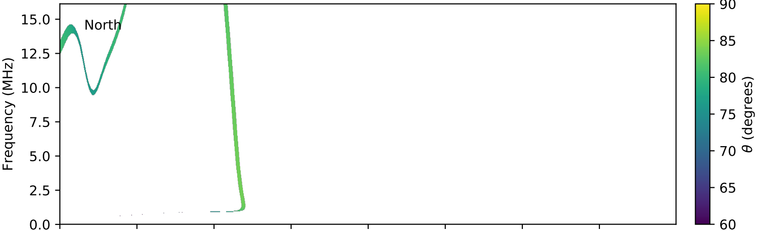
expres_cassini_jupiter_europa_isaac_lossc-wid1deg_3kev_20020802_v01.cdf
