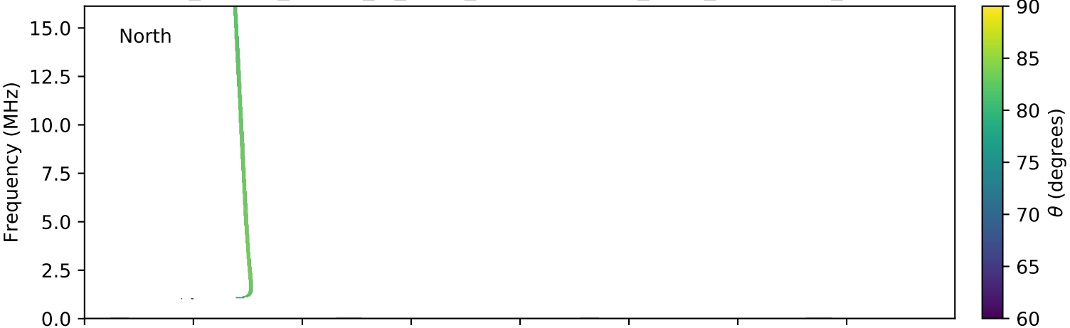
expres_cassini_jupiter_io_isaac_lossc-wid1deg_3kev_20020724_v01.cdf
