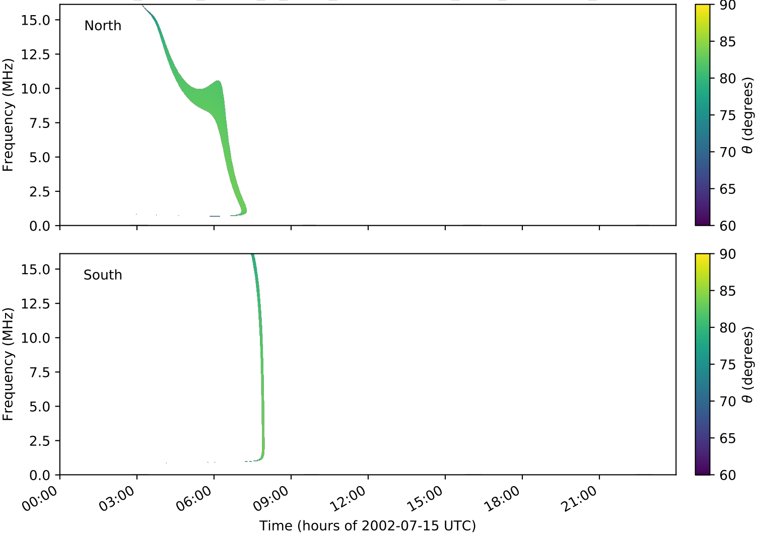
expres_cassini_jupiter_io_isaac_lossc-wid1deg_3kev_20020715_v01.cdf
