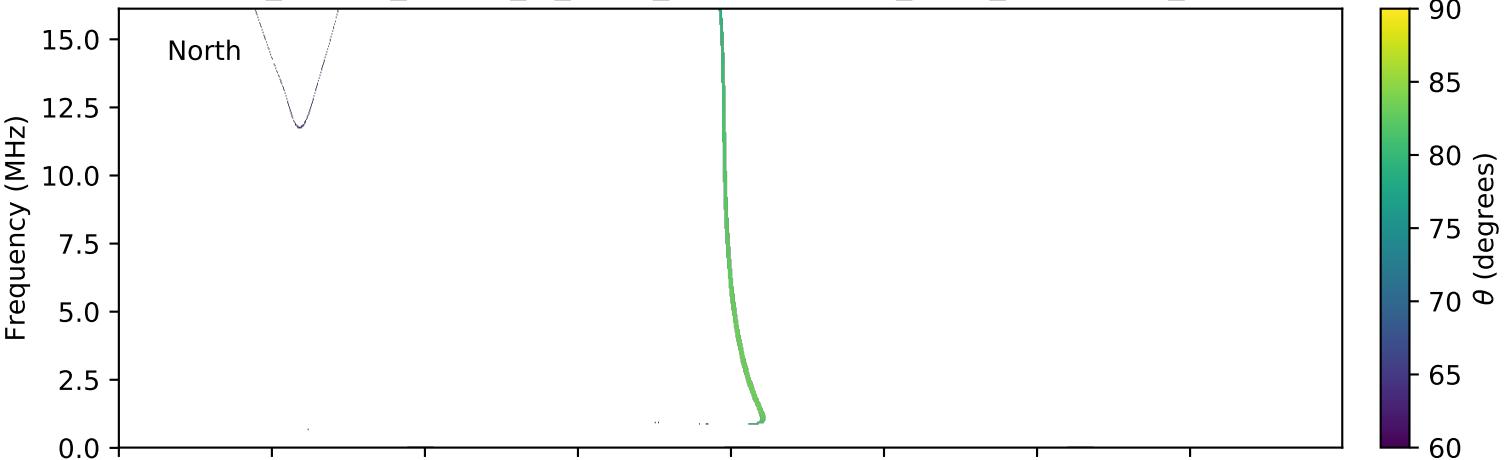
expres_cassini_jupiter_io_isaac_lossc-wid1deg_3kev_20020713_v01.cdf
