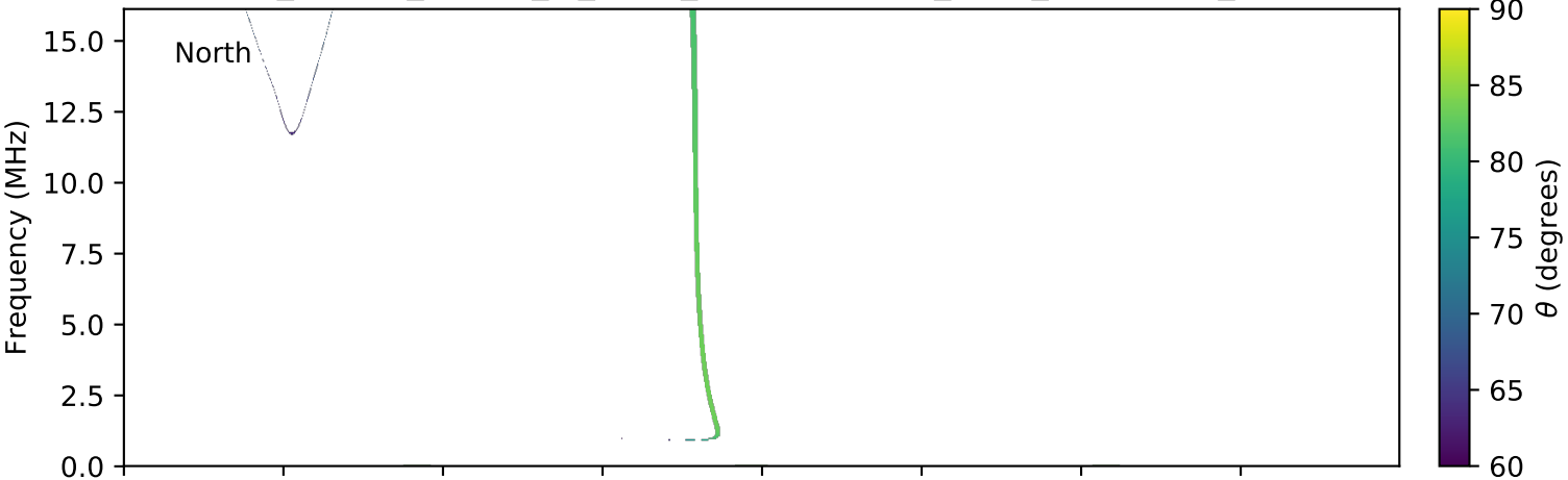
expres_cassini_jupiter_io_isaac_lossc-wid1deg_3kev_20020706_v01.cdf
