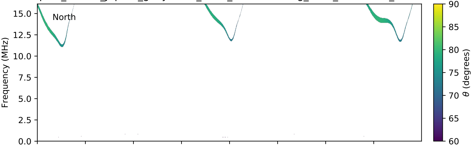
expres_cassini_jupiter_ganymede_isaac_lossc-wid1deg_3kev_20020730_v01.cdf
