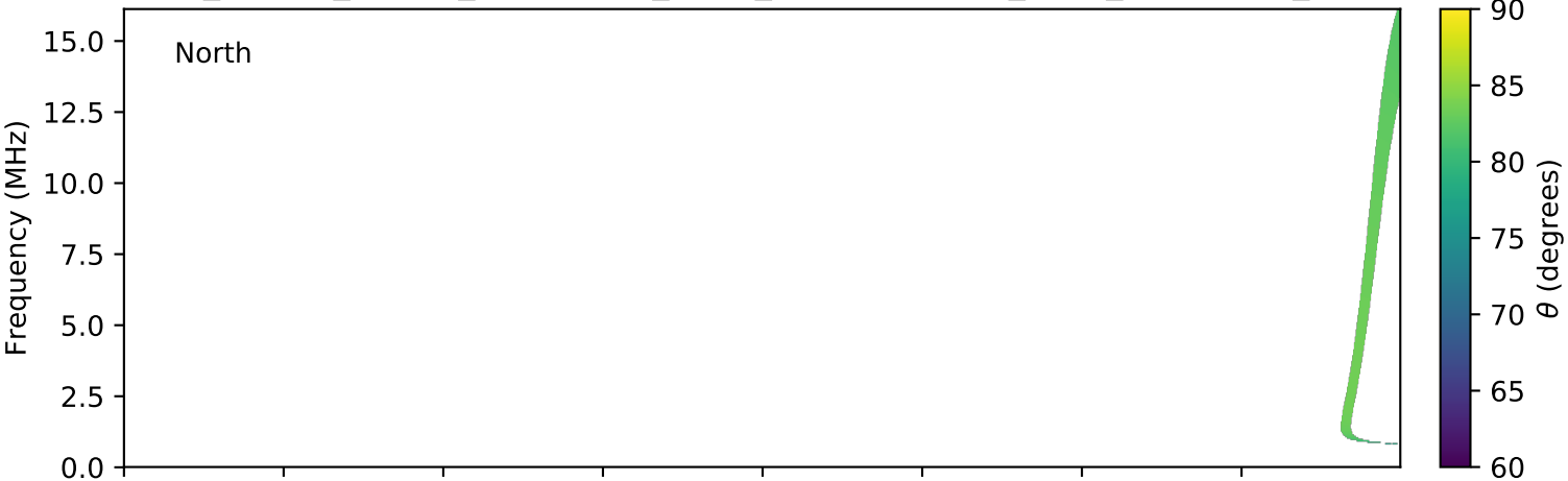
expres_cassini_jupiter_ganymede_isaac_lossc-wid1deg_3kev_20020728_v01.cdf
