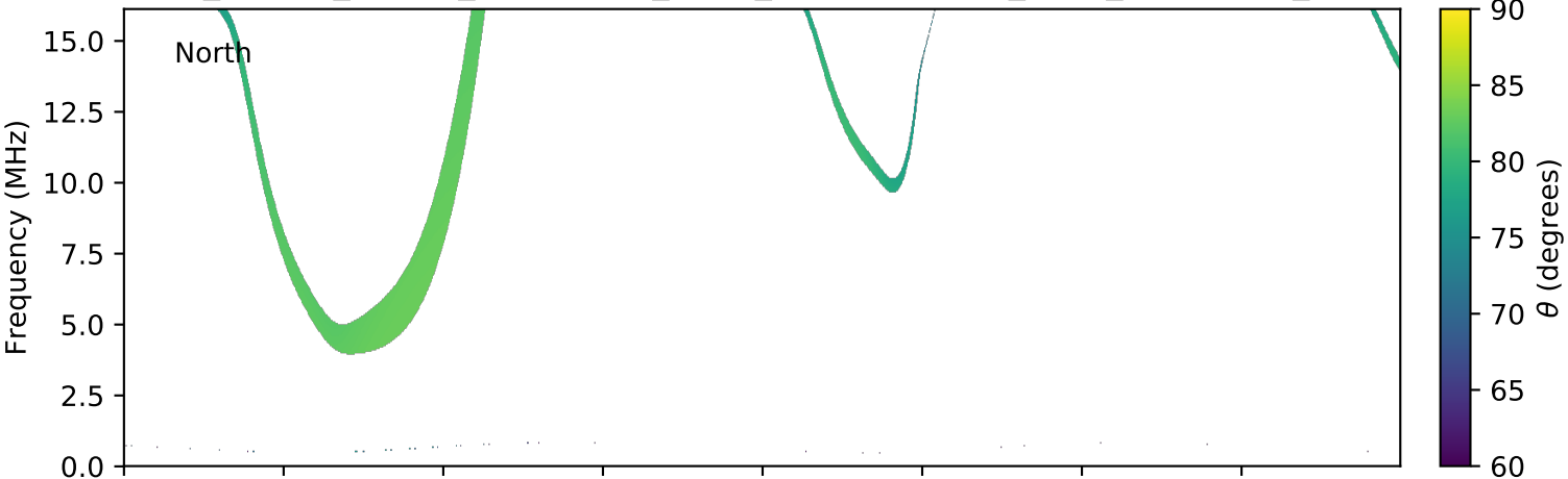
expres_cassini_jupiter_ganymede_isaac_lossc-wid1deg_3kev_20020722_v01.cdf
