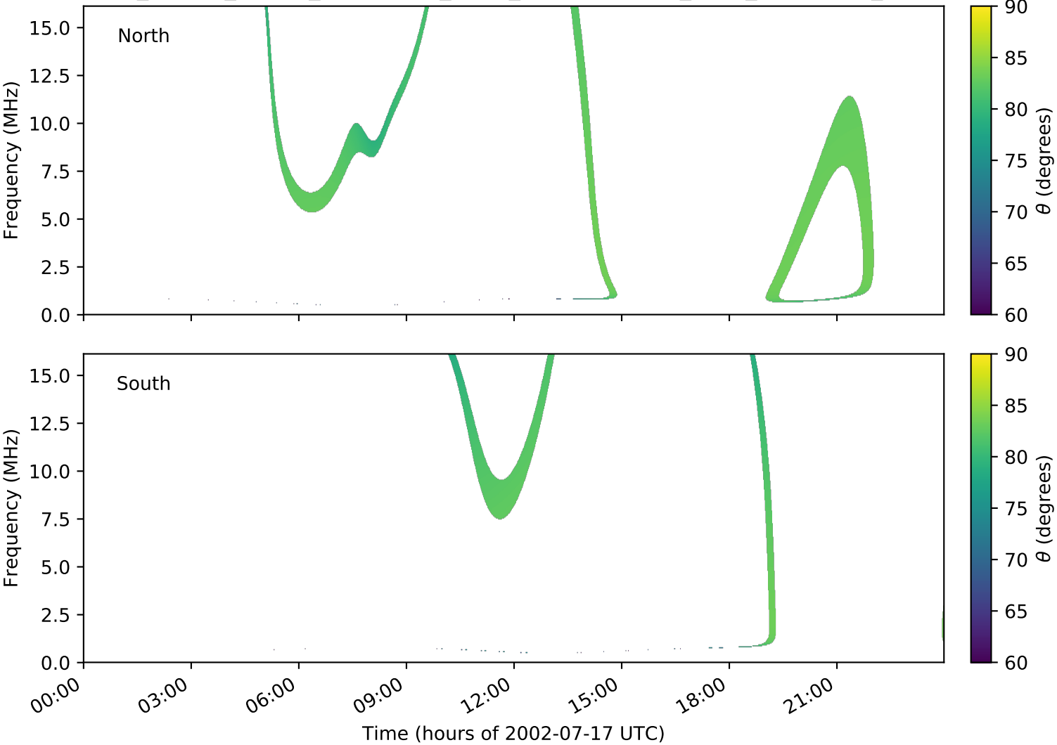
expres_cassini_jupiter_ganymede_isaac_lossc-wid1deg_3kev_20020717_v01.cdf
