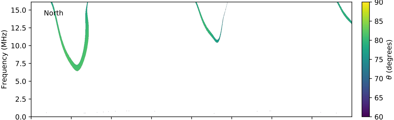
expres_cassini_jupiter_ganymede_isaac_lossc-wid1deg_3kev_20020715_v01.cdf
