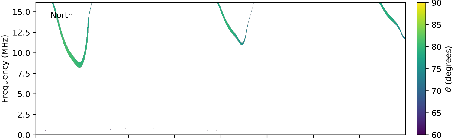
expres_cassini_jupiter_ganymede_isaac_lossc-wid1deg_3kev_20020708_v01.cdf
