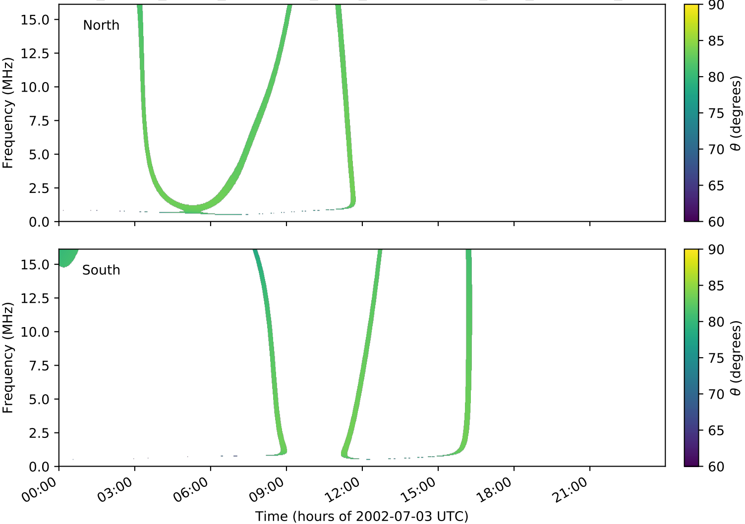
expres_cassini_jupiter_ganymede_isaac_lossc-wid1deg_3kev_20020703_v01.cdf
