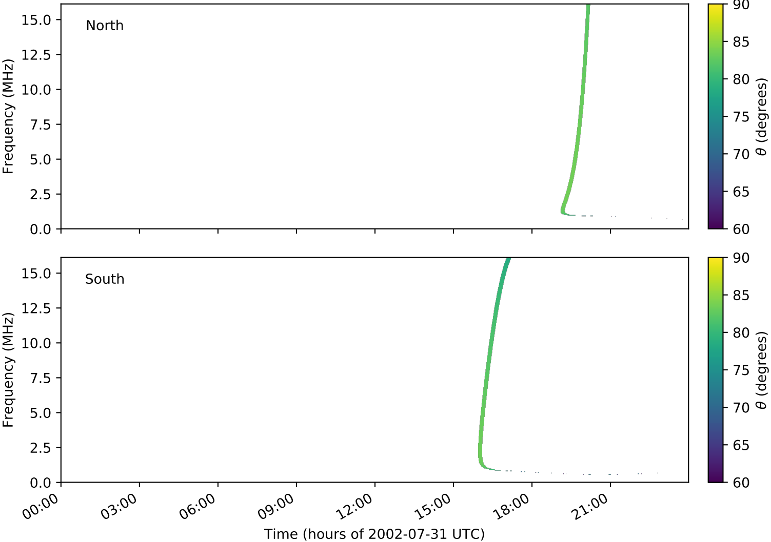
expres_cassini_jupiter_europa_isaac_lossc-wid1deg_3kev_20020731_v01.cdf
