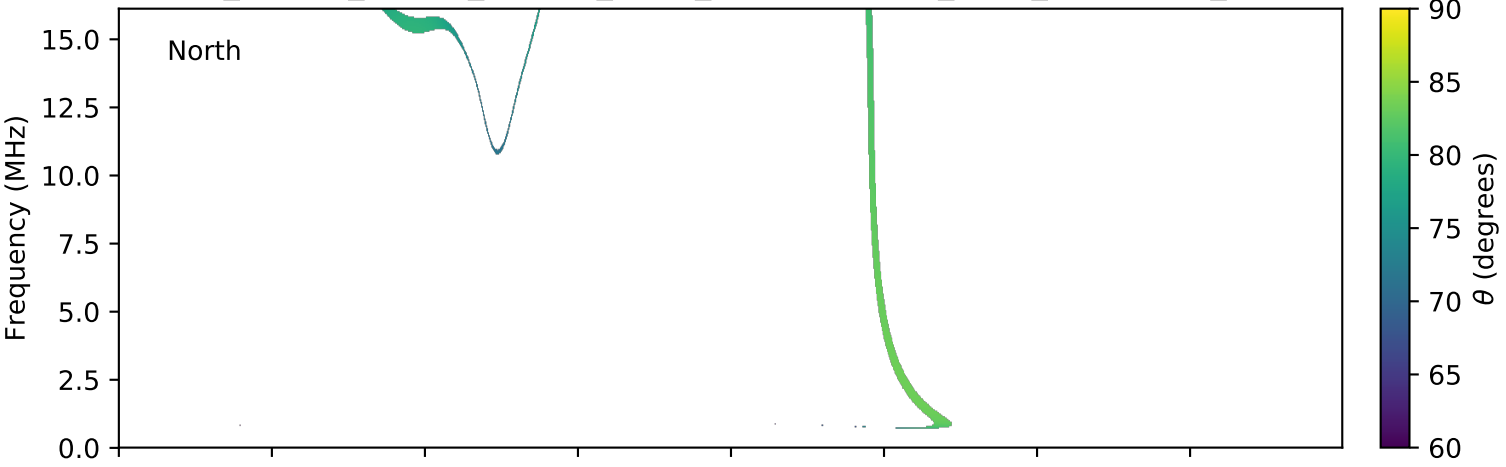
expres_cassini_jupiter_europa_isaac_lossc-wid1deg_3kev_20020729_v01.cdf
