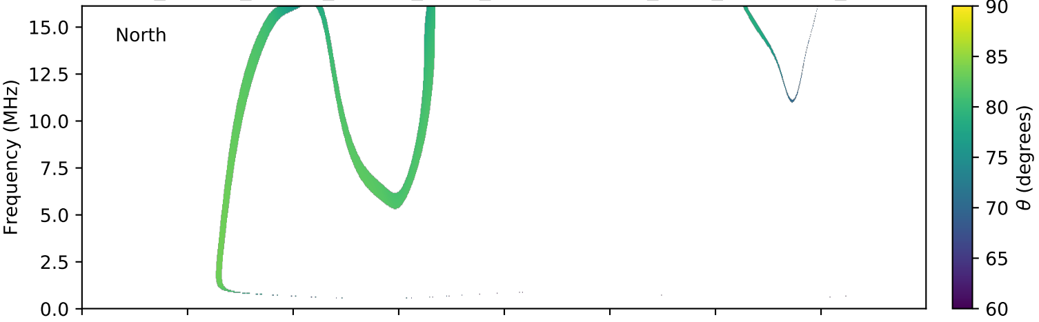
expres_cassini_jupiter_europa_isaac_lossc-wid1deg_3kev_20020728_v01.cdf
