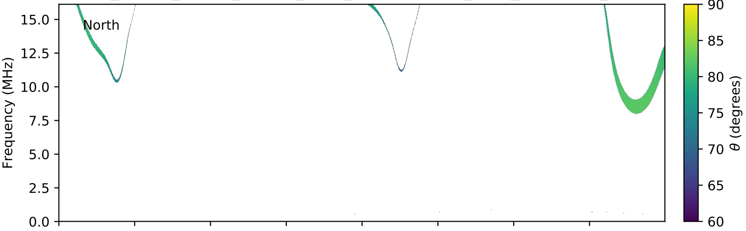
expres_cassini_jupiter_europa_isaac_lossc-wid1deg_3kev_20020725_v01.cdf
