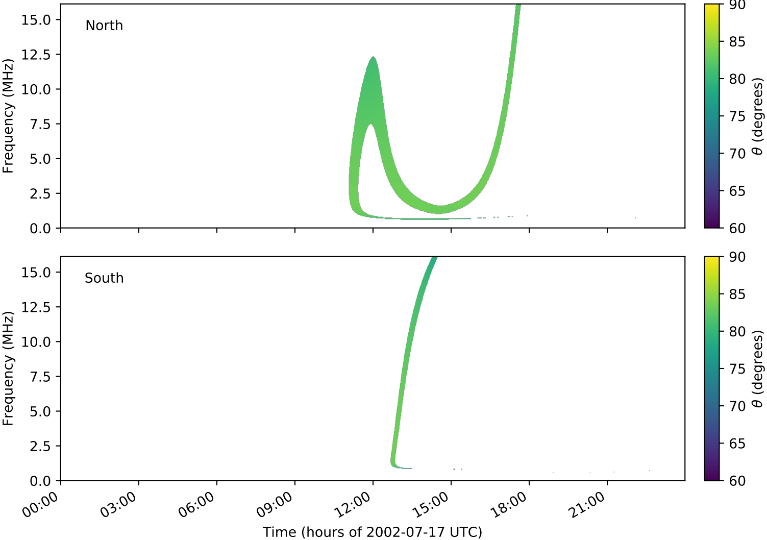
expres_cassini_jupiter_europa_isaac_lossc-wid1deg_3kev_20020717_v01.cdf
