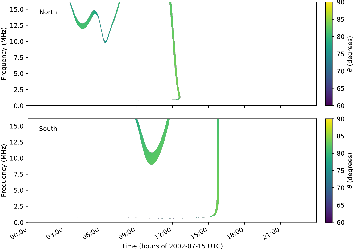
expres_cassini_jupiter_europa_isaac_lossc-wid1deg_3kev_20020715_v01.cdf
