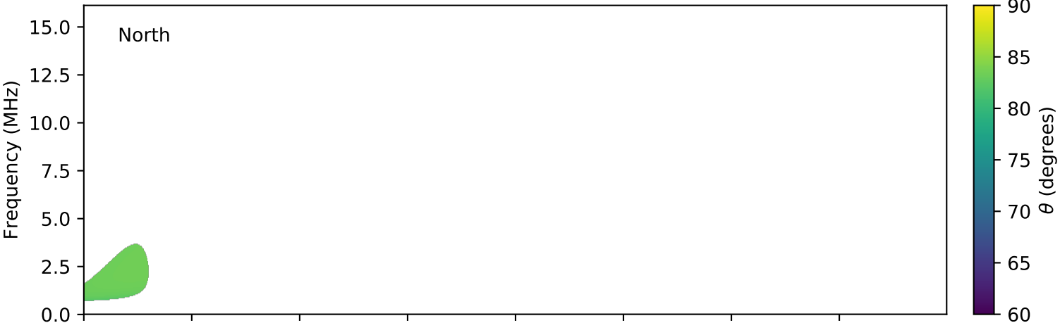
expres_cassini_jupiter_europa_isaac_lossc-wid1deg_3kev_20020712_v01.cdf
