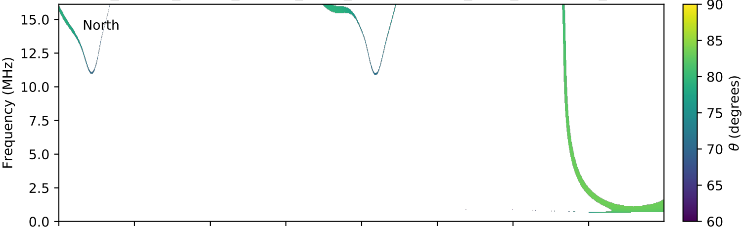
expres_cassini_jupiter_europa_isaac_lossc-wid1deg_3kev_20020711_v01.cdf
