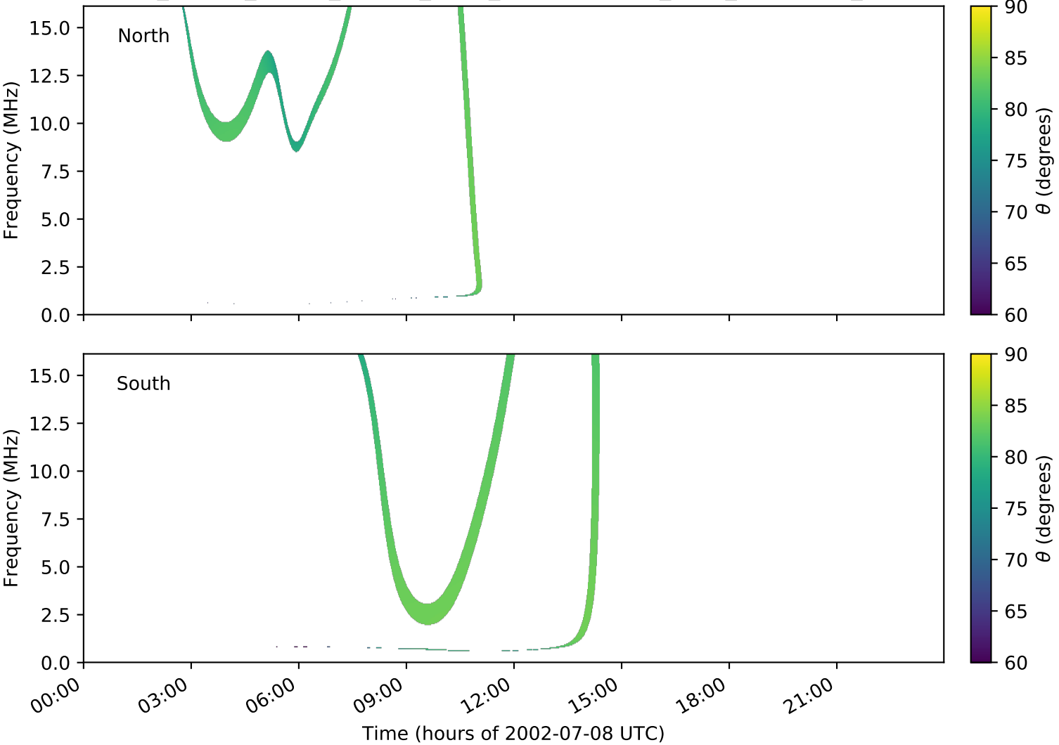
expres_cassini_jupiter_europa_isaac_lossc-wid1deg_3kev_20020708_v01.cdf
