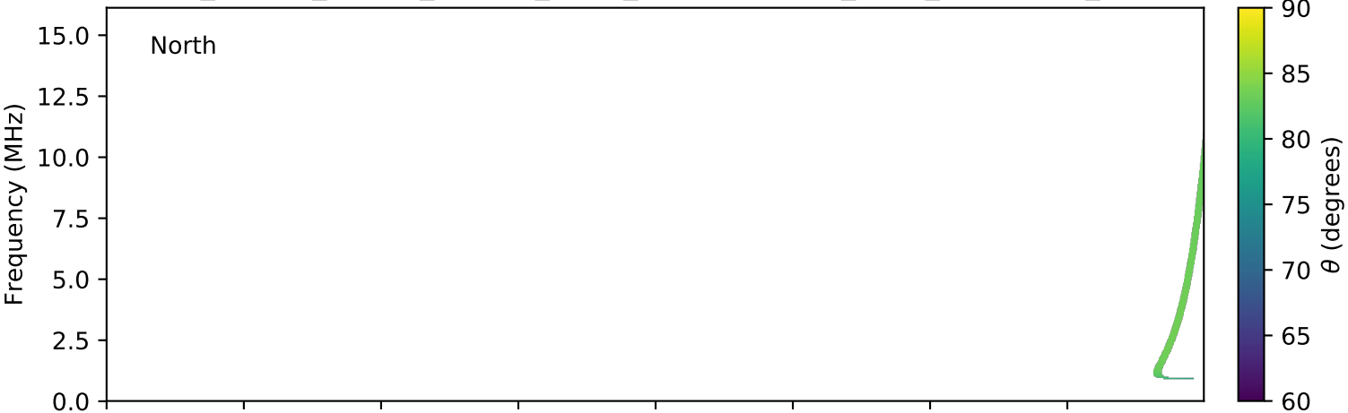
expres_cassini_jupiter_europa_isaac_lossc-wid1deg_3kev_20020706_v01.cdf
