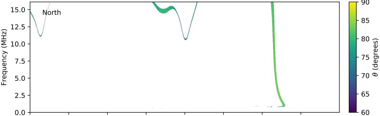
expres_cassini_jupiter_europa_isaac_lossc-wid1deg_3kev_20020704_v01.cdf
