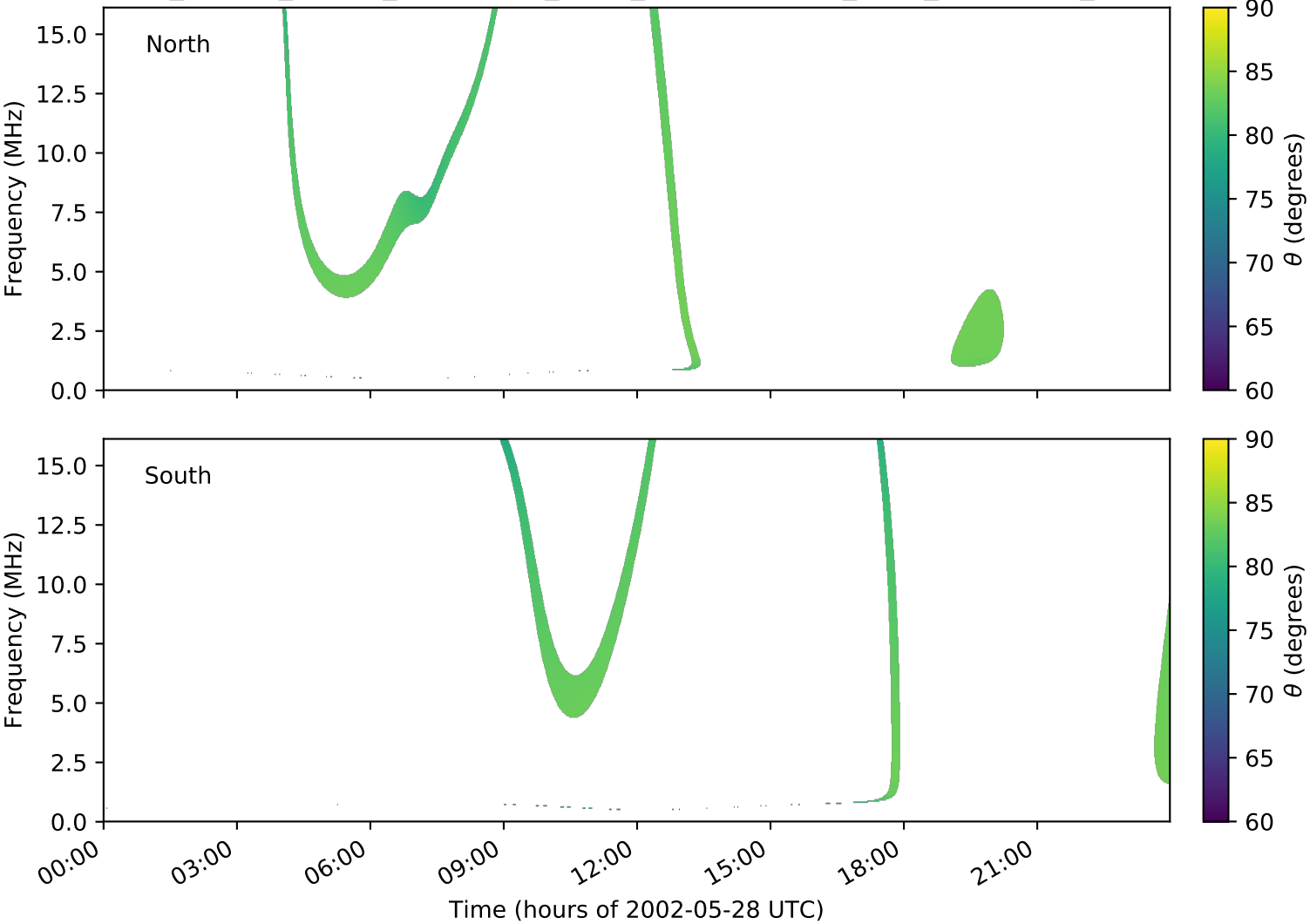
expres_cassini_jupiter_ganymede_isaac_lossc-wid1deg_3kev_20020528_v01.cdf
