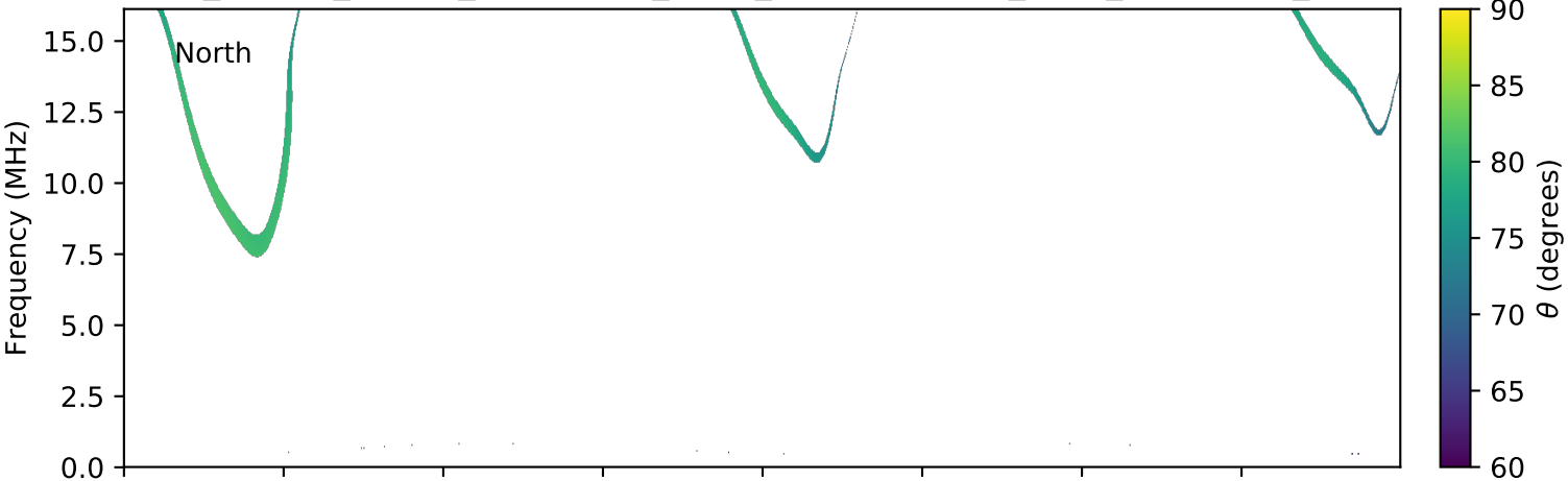
expres_cassini_jupiter_ganymede_isaac_lossc-wid1deg_3kev_20020526_v01.cdf
