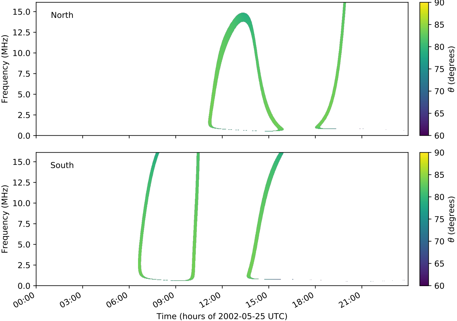
expres_cassini_jupiter_ganymede_isaac_lossc-wid1deg_3kev_20020525_v01.cdf
