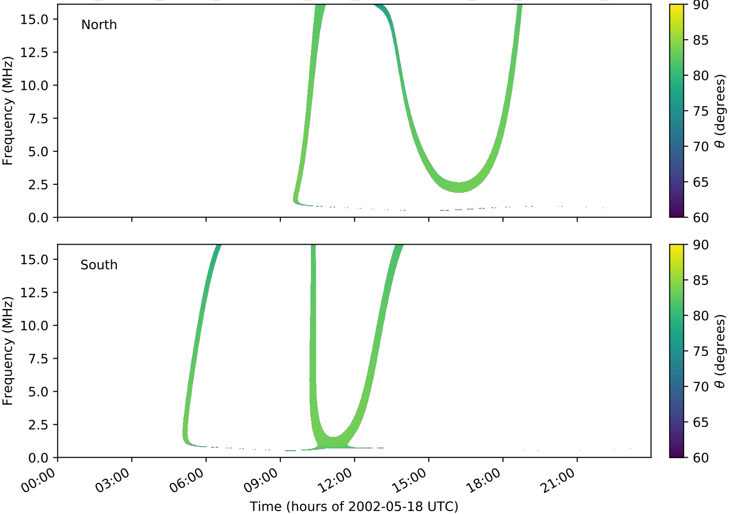
expres_cassini_jupiter_ganymede_isaac_lossc-wid1deg_3kev_20020518_v01.cdf
