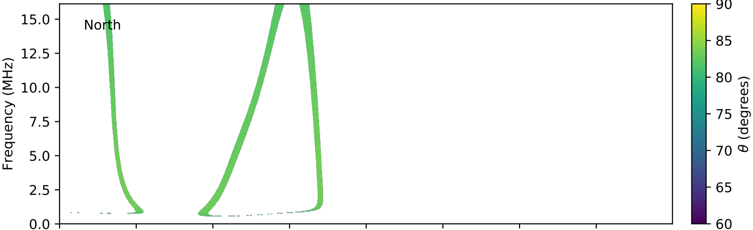
expres_cassini_jupiter_ganymede_isaac_lossc-wid1deg_3kev_20020514_v01.cdf
