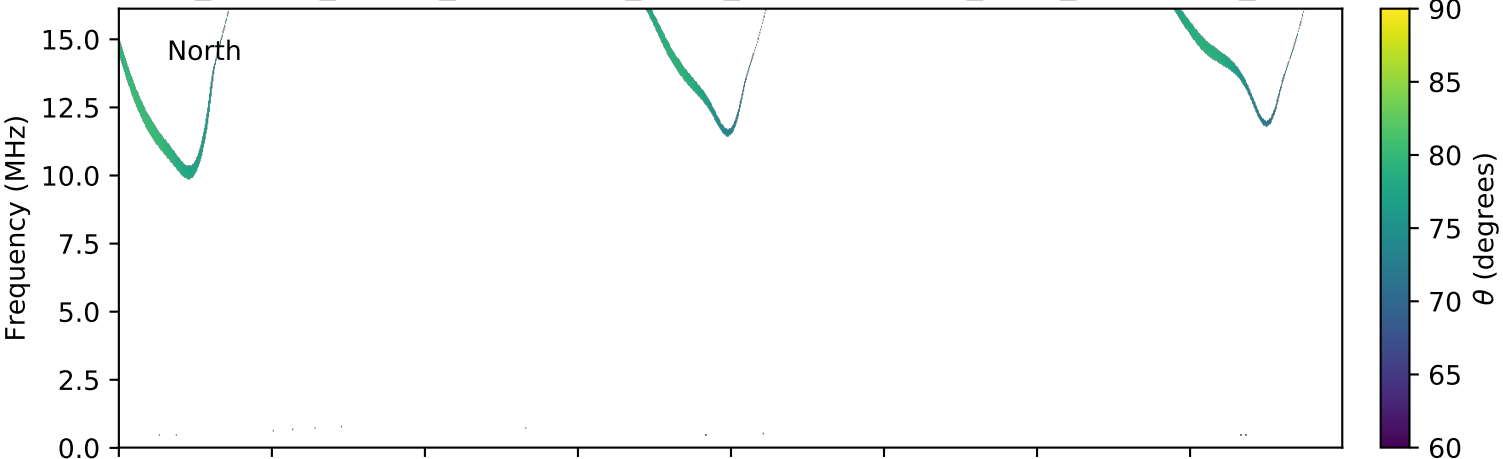
expres_cassini_jupiter_ganymede_isaac_lossc-wid1deg_3kev_20020512_v01.cdf
