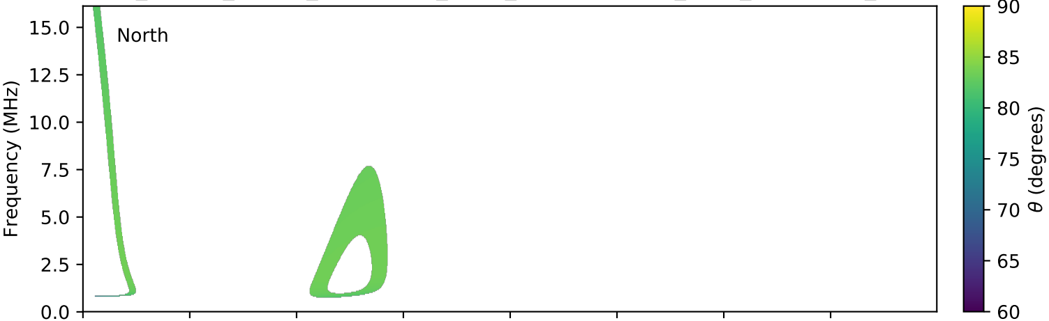
expres_cassini_jupiter_ganymede_isaac_lossc-wid1deg_3kev_20020507_v01.cdf
