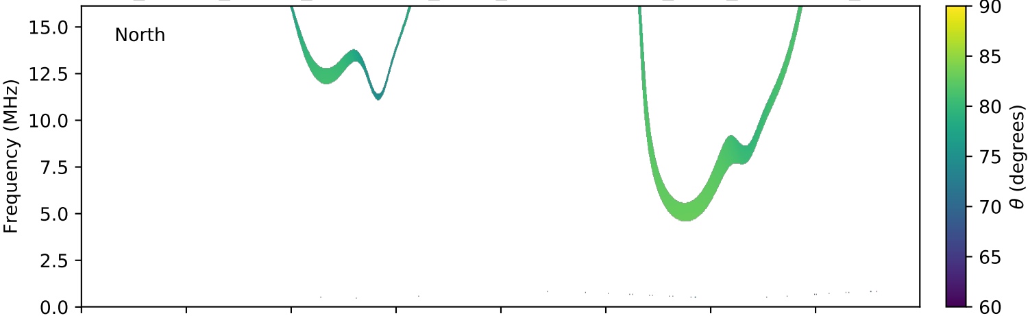
expres_cassini_jupiter_ganymede_isaac_lossc-wid1deg_3kev_20020506_v01.cdf
