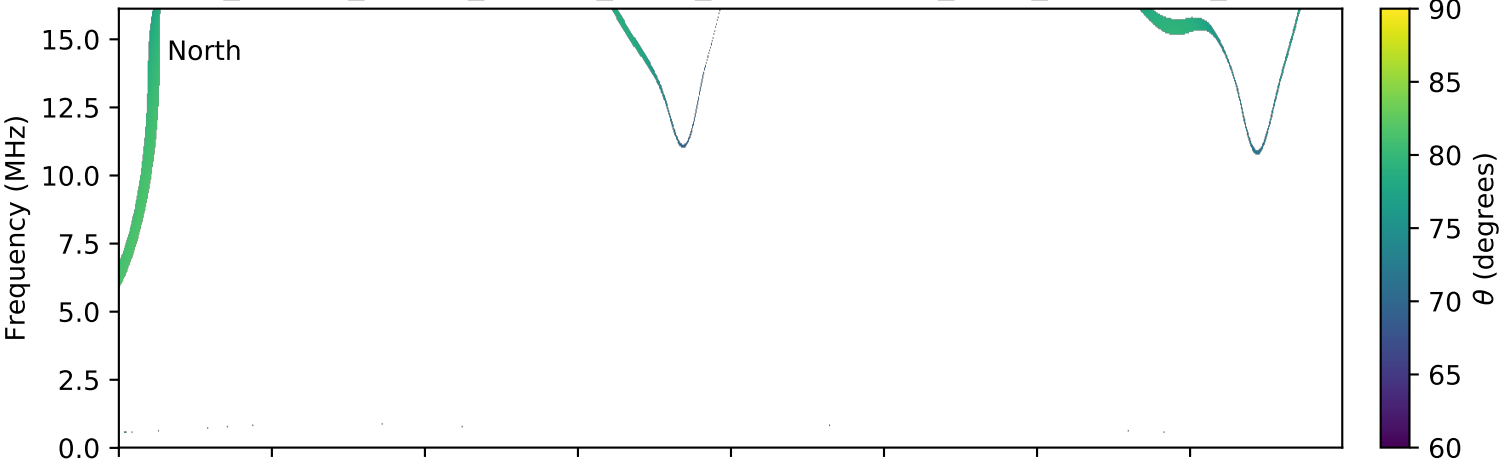
expres_cassini_jupiter_europa_isaac_lossc-wid1deg_3kev_20020529_v01.cdf
