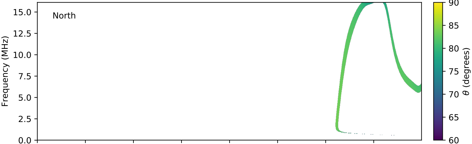
expres_cassini_jupiter_europa_isaac_lossc-wid1deg_3kev_20020528_v01.cdf
