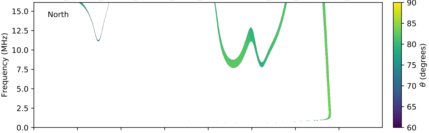
expres_cassini_jupiter_europa_isaac_lossc-wid1deg_3kev_20020526_v01.cdf
