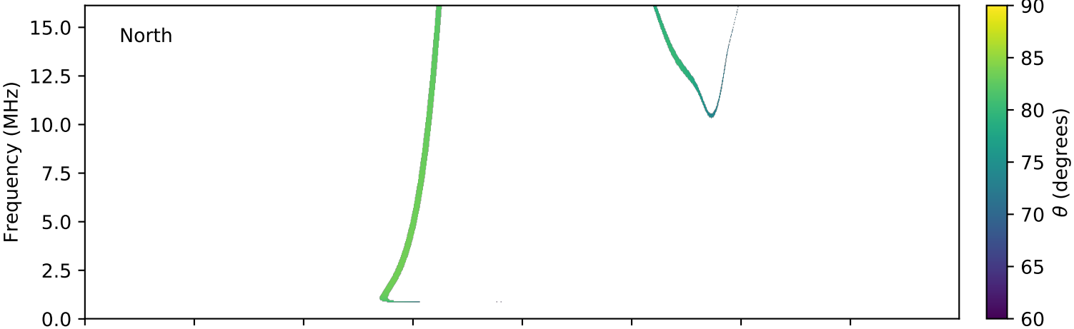
expres_cassini_jupiter_europa_isaac_lossc-wid1deg_3kev_20020525_v01.cdf
