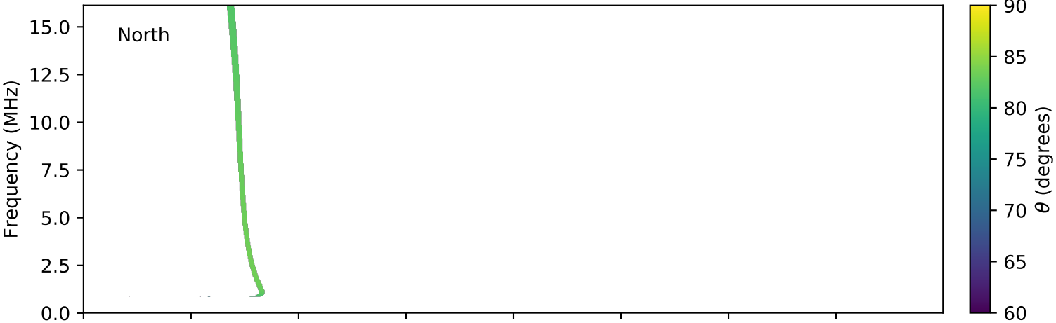
expres_cassini_jupiter_europa_isaac_lossc-wid1deg_3kev_20020523_v01.cdf
