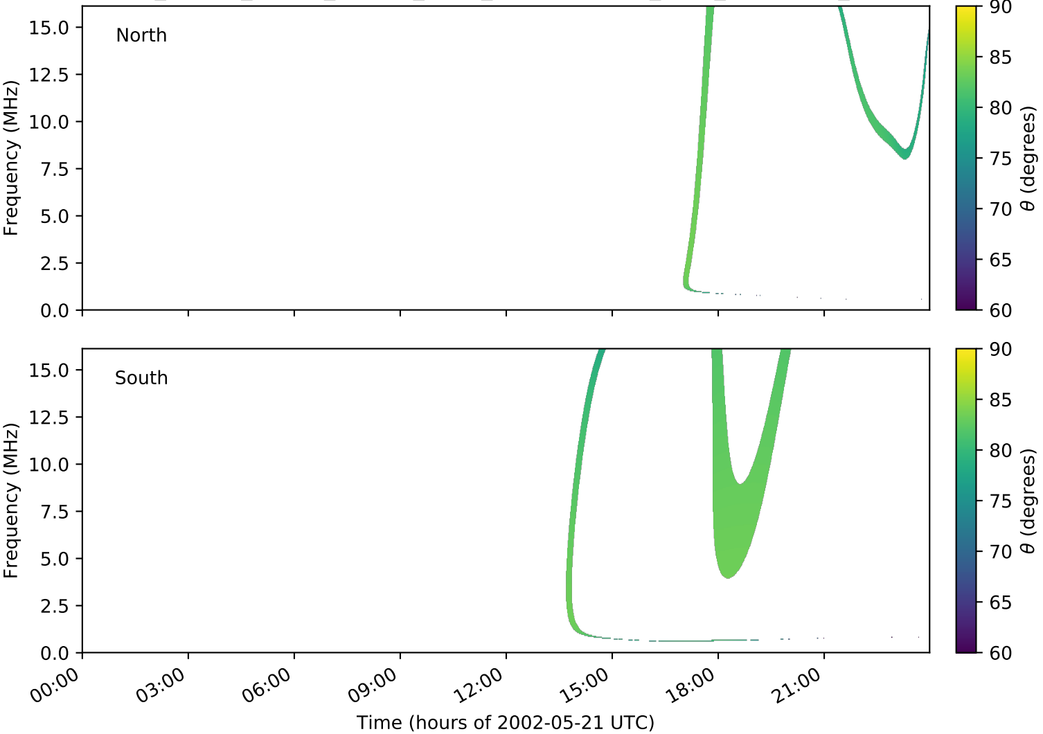
expres_cassini_jupiter_europa_isaac_lossc-wid1deg_3kev_20020521_v01.cdf
