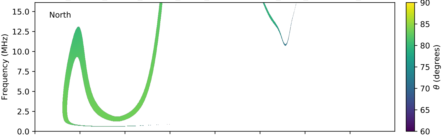
expres_cassini_jupiter_europa_isaac_lossc-wid1deg_3kev_20020518_v01.cdf
