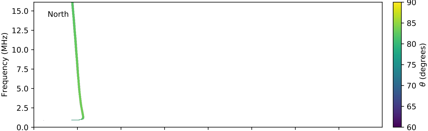
expres_cassini_jupiter_europa_isaac_lossc-wid1deg_3kev_20020516_v01.cdf
