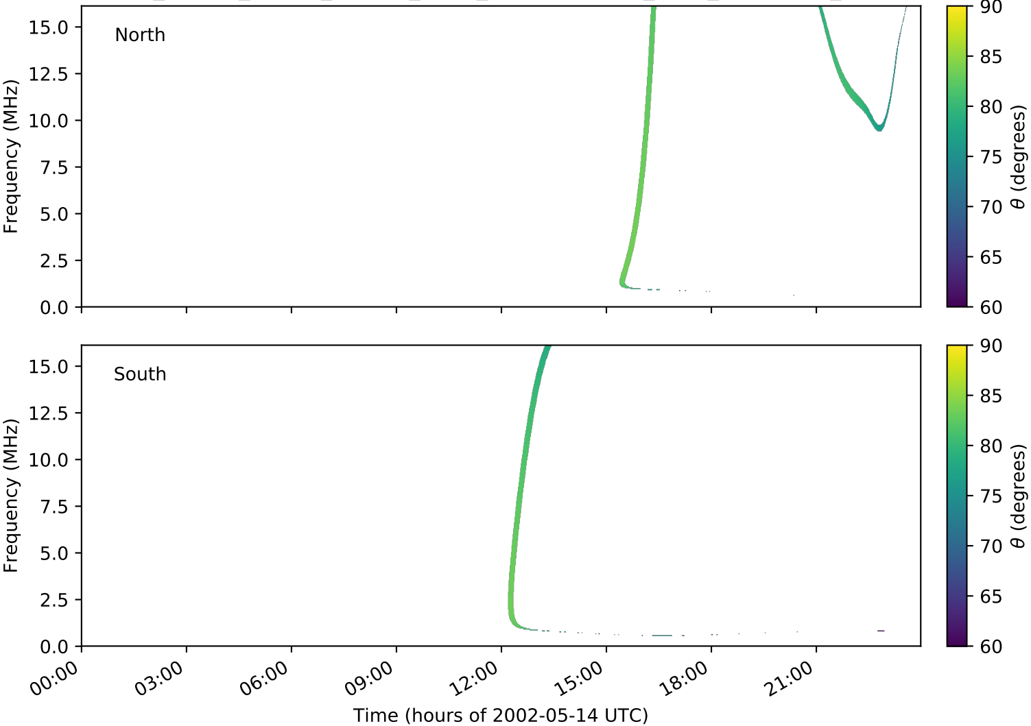
expres_cassini_jupiter_europa_isaac_lossc-wid1deg_3kev_20020514_v01.cdf
