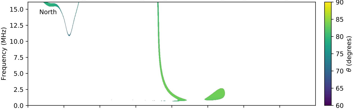
expres_cassini_jupiter_europa_isaac_lossc-wid1deg_3kev_20020512_v01.cdf
