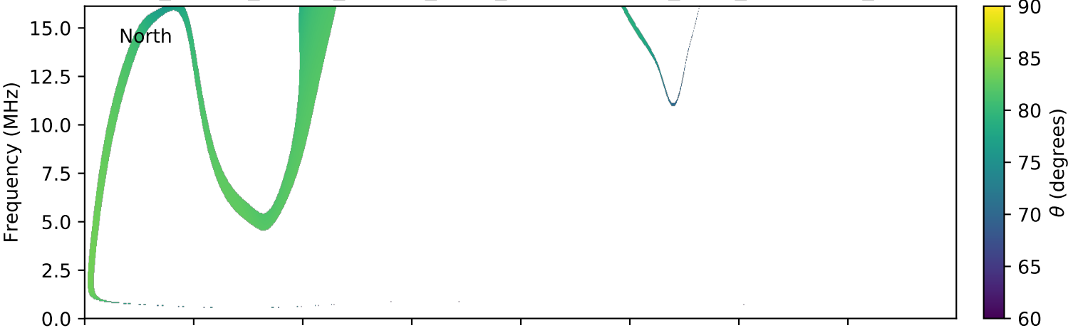
expres_cassini_jupiter_europa_isaac_lossc-wid1deg_3kev_20020511_v01.cdf
