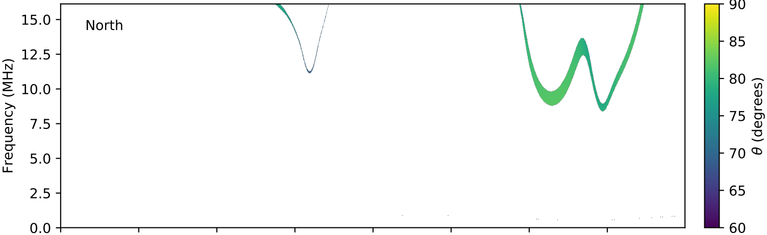
expres_cassini_jupiter_europa_isaac_lossc-wid1deg_3kev_20020508_v01.cdf
