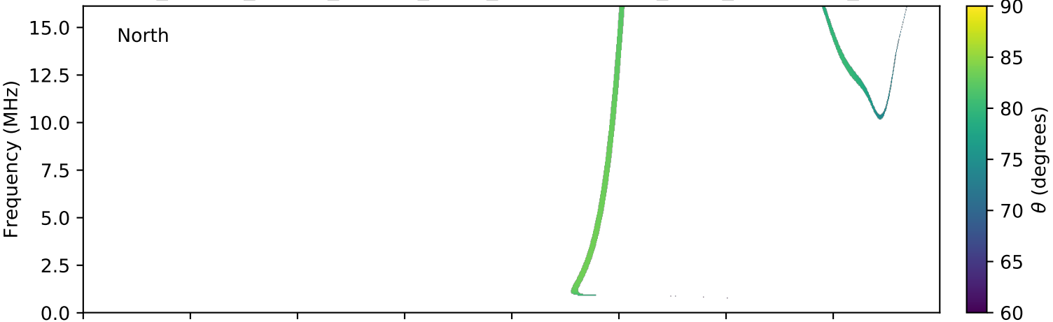
expres_cassini_jupiter_europa_isaac_lossc-wid1deg_3kev_20020507_v01.cdf
