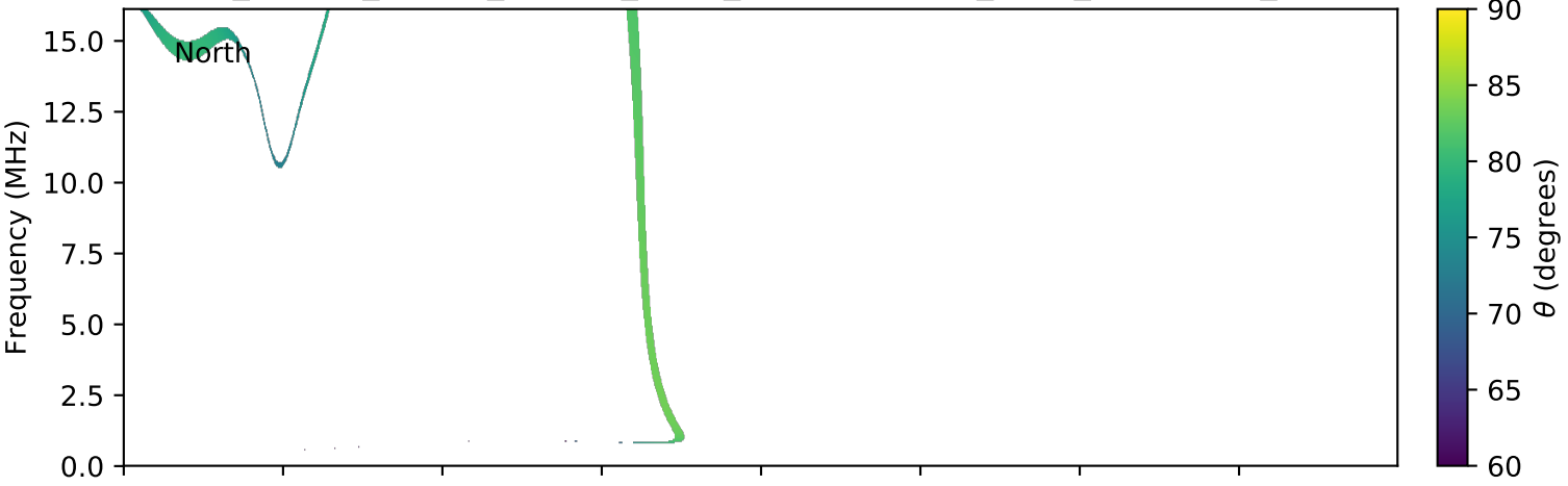
expres_cassini_jupiter_europa_isaac_lossc-wid1deg_3kev_20020505_v01.cdf
