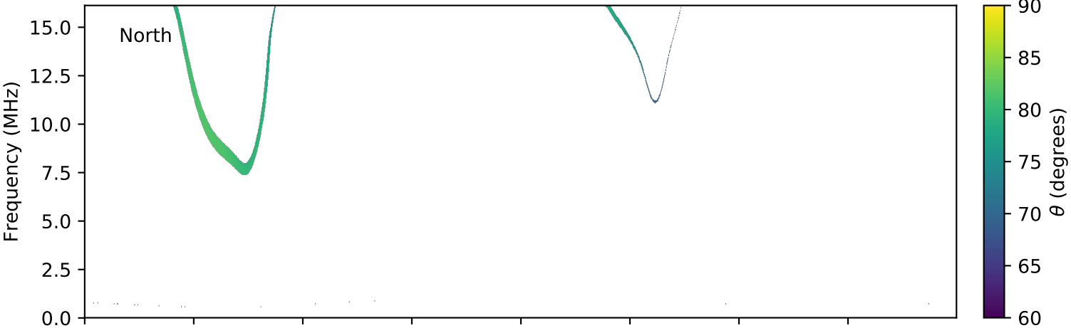
expres_cassini_jupiter_europa_isaac_lossc-wid1deg_3kev_20020504_v01.cdf
